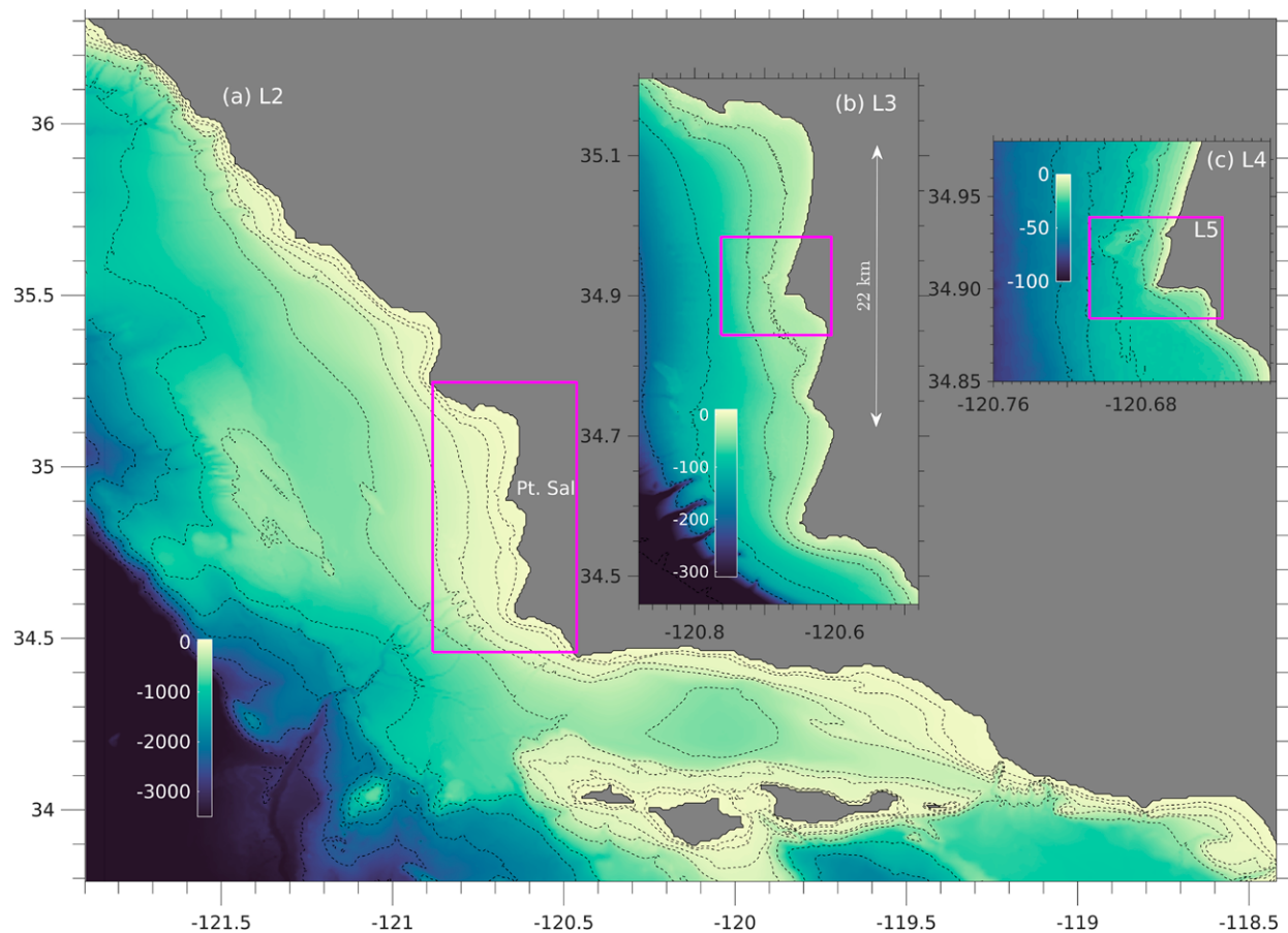
Fig. 5. Nested Regional Ocean Modeling System grids (L2, L3, L4, L5) and observation locations: (a) second-level nested grid (L2, resolution: 600 m). Color bar is the water depth h in meters; (b) L3 grid (resolution: 200 m), and (c) L4 grid (resolution: 66 m). In (a) dashed black lines are depth contours of 30, 50, 100, 200, 500, 1,000, 1,500, 2,000, 2,500, and 3,000 m. Parent grids L0 and L1 are shown elsewhere (Suanda et al. 2016).
