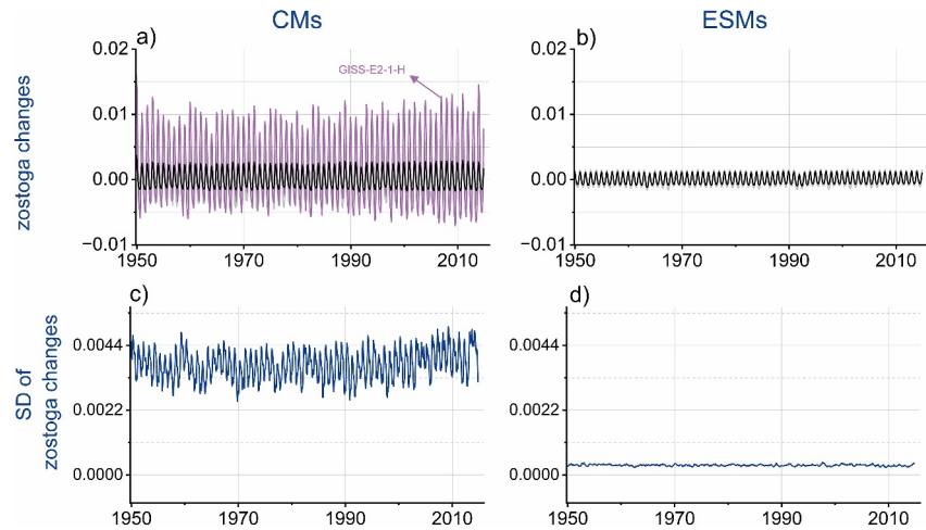
Figure 2. Comparison between global-mean thermosteric sea-level change ( h_\theta ) as estimated by (a) climate models (CMs) and (b) earth system models (ESMs). The standard deviation of h_\theta changes among CMs and ESMs is shown in panels (c, d).
