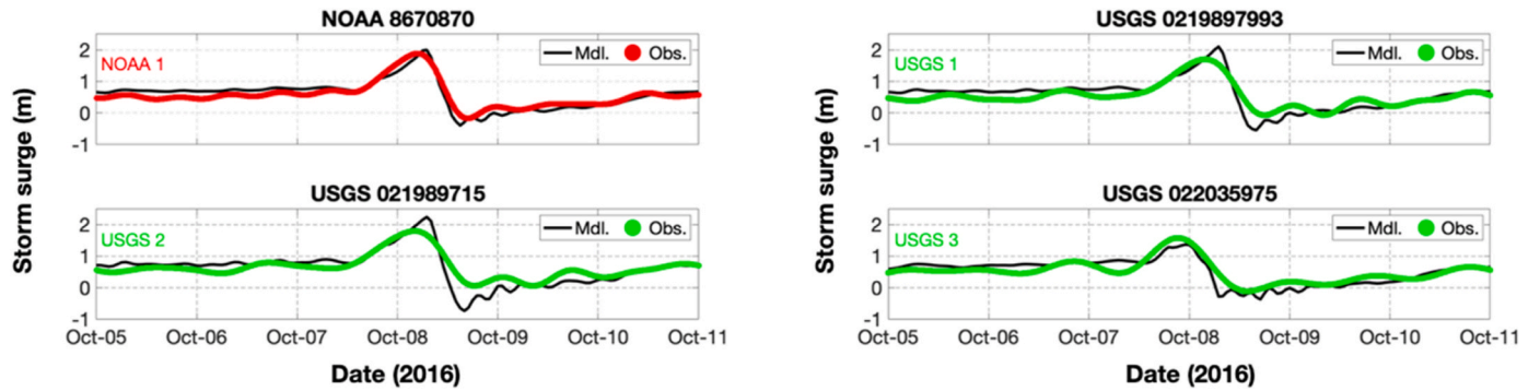
Fig. 10. The comparison of storm surge between model and observations during Hurricanes Matthew at different locations (NOAA and USGS) indicated in Fig. 7. Color code is used to indicate the different observations such as NOAA (red) and USGS (green).
