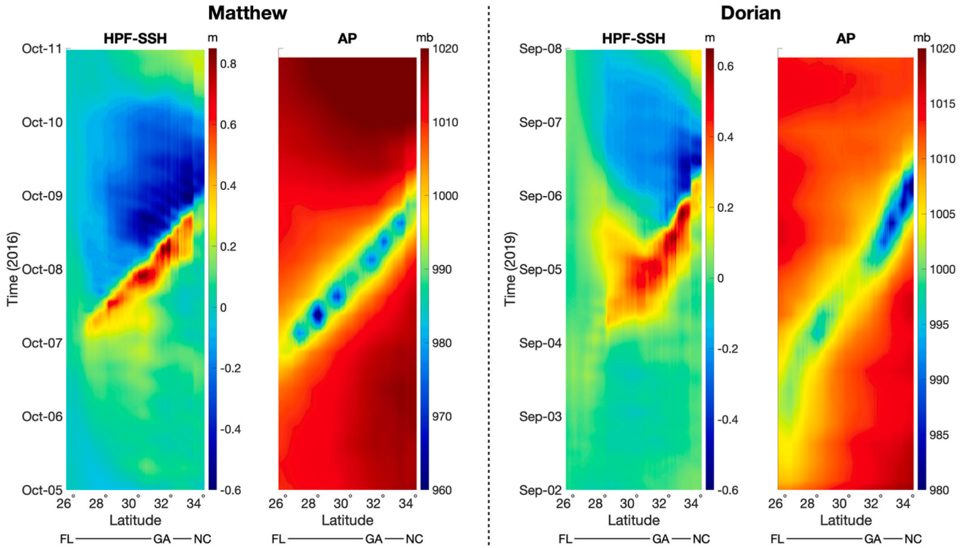
Fig. 6. Hovmöller (latitude-time) diagram of the High-Pass Filtered Sea Surface Height (HPF SSH) and atmospheric pressure (AP) during Hurricanes Matthew (left two columns) and Dorian (right two columns). The latitude in x-axis follows the coastline from Florida (FL) to Georgia (GA) and North Carolina (NC).
