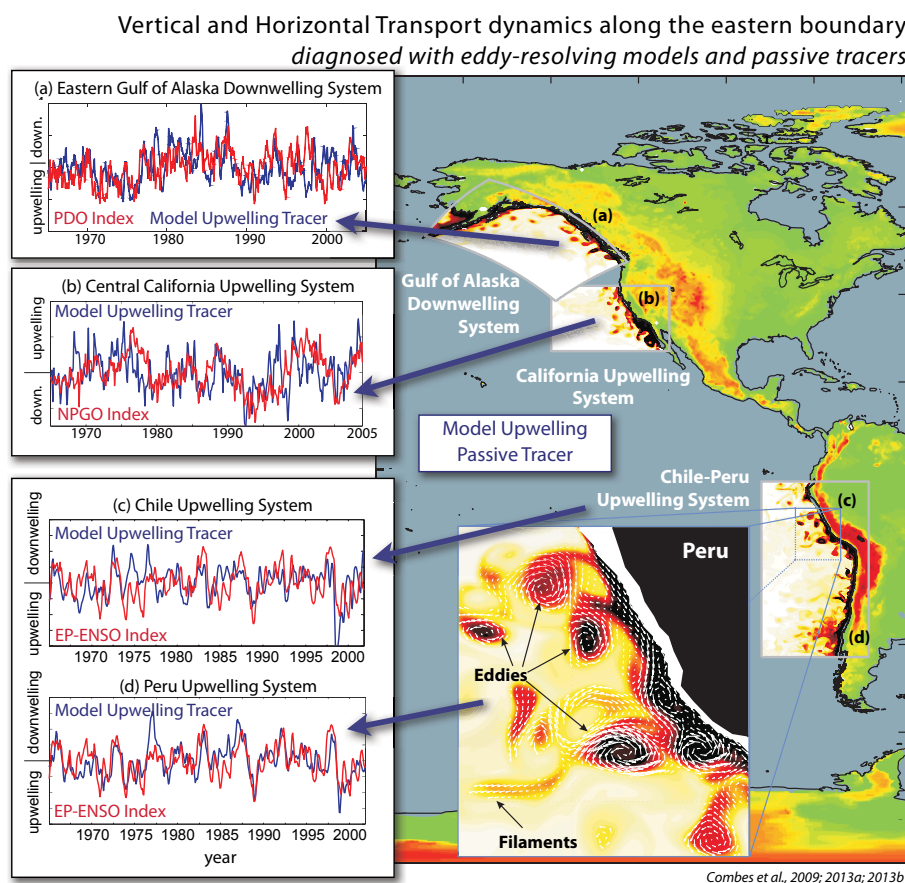
Figure 5. Regional Ocean Modeling System (ROMS) passive tracer transport experiments. Map showing a February 1998 snapshot of passive tracers released from the coast in the nested eddy-resolving ROMS hindcast from 1950 to 2008. The passive tracers were used to study ocean transport dynamics in each of the POBEX regions. The time series panels show how indices of upwelling defined from the passive tracers are linked to different Pacific climate indices in the different POBEX regions (see Combes et al., 2009 and 2013, for details on definitions).
