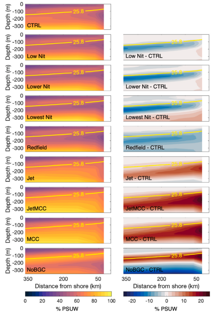
Fig. 3. Vertical sections of the (left) annual mean PSUW content for the CTRL and sensitivity experiments and (right) the difference in %PSUW between the sensitivity experiments and the CTRL along Line 80. Yellow lines represent the 25.8 isopycnal surface. (For interpretation of the references to colour in this figure legend, the reader is referred to the Web version of this article.)
