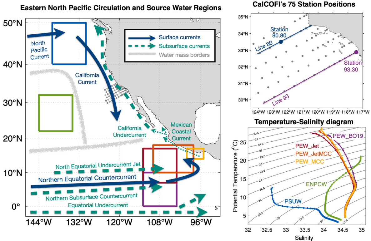
Fig. 1. (left) Schematic of eastern North Pacific showing the source water regions for Pacific Subarctic Upper Water (PSUW; blue box), Eastern North Pacific Central Water (ENPCW; green box), and Pacific Equatorial Water (PEW BO19 ; purple box), the proposed PEW source regions for the sensitivity experiments: Jet (red box), JetMCC (orange box), and MCC (yellow box). The dominant surface and subsurface currents are also shown. (top right) Nominal CalCOFI grid showing stations. Lines 80 and 93, and stations 80.80 and 93.30 are labeled. (bottom right) Temperature-salinity diagram for PSUW (blue), ENPCW (green), PEW BO19 (purple), PEW Jet (red), PEW JetMCC (orange), PEW MCC (yellow). Data obtained from the World Ocean Database (WOD18) for the period 1984–2017. (For interpretation of the references to colour in this figure legend, the reader is referred to the Web version of this article.)
