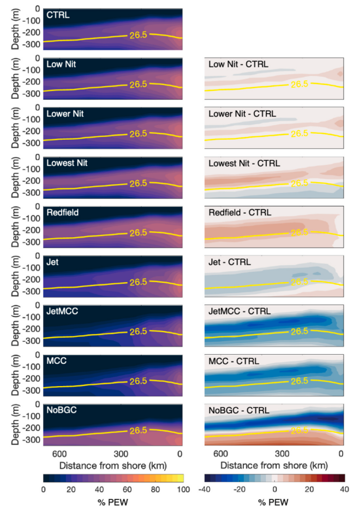
Fig. 5. Vertical sections of the (left) annual mean PEW content for the CTRL and sensitivity experiments and (right) the difference in %PEW between the sensitivity experiments and the CTRL along Line 93. Yellow lines represent the 26.5 isopycnal surface. (For interpretation of the references to colour in this figure legend, the reader is referred to the Web version of this article.)
