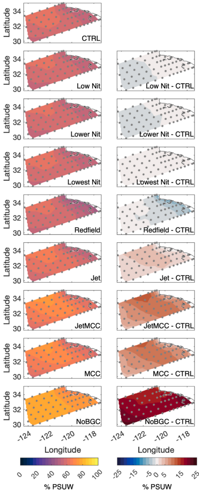
Fig. 2. Maps of the (left) annual mean PSUW content for the CTRL and sensitivity experiments and (right) the difference in %PSUW between the sensitivity experiments and the CTRL on the 25.8 isopycnal surface. Grey dots represent the location of the CalCOFI stations.
