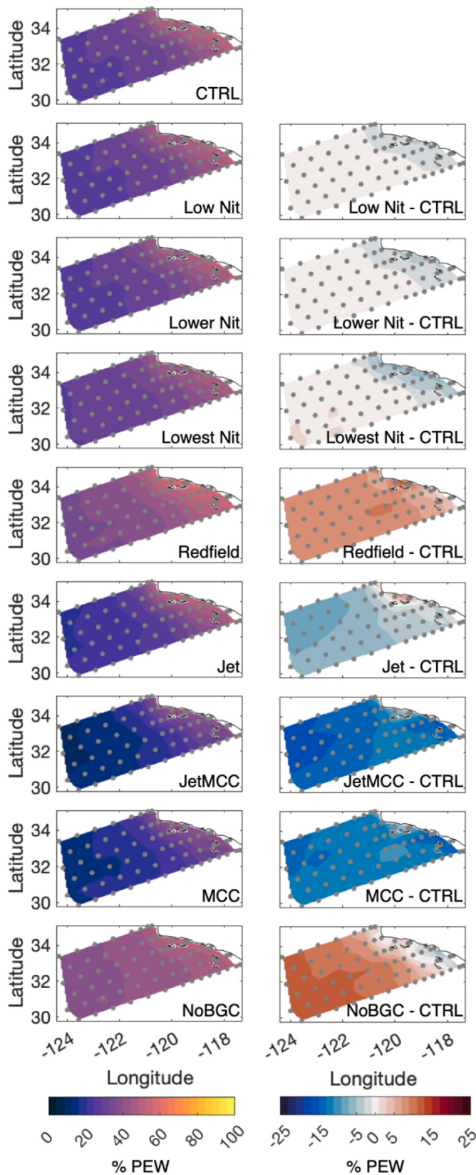
Fig. 4. Maps of the (left) annual mean PEW content for the CTRL and sensitivity experiments and (right) the difference in %PEW between the sensitivity experiments and the CTRL on the 26.5 isopycnal surface. Grey dots represent the location of the CalCOFI stations.
