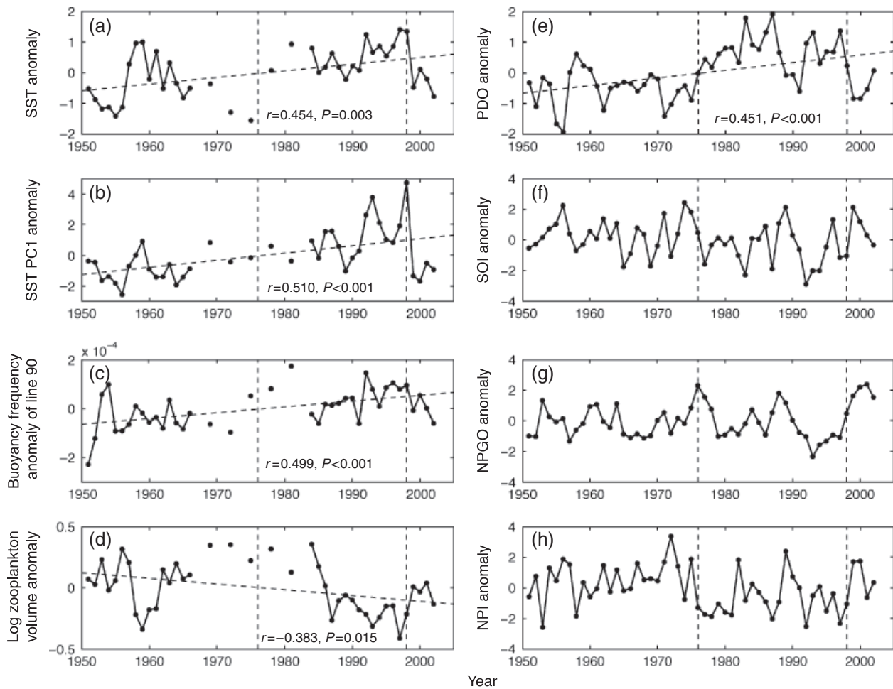
Fig. 3 Time series anomalies of local environmental variables: (a) sea surface temperature (SST), (b) first principal component of spatial SST, (c) average buoyancy frequency at the pycnocline depth for the line 90, and (d) zooplankton displacement volume for the studied area (sensu Fig. 1), and large-scale climate indices: (e) Pacific Decadal Oscillation, (f) Southern Oscillation Index, (g) North Pacific Gyre Oscillation, and (h) North Pacific Index. Note that for the local variables, sampling was triennial from 1966 to 1984. If a time series exhibited a significant long-term trend, a trend line (the dashed line) is shown along with the coefficient of correlation and P -value. The two vertical dashed lines indicate years of change of climate regimes. PC1, first principal component.
