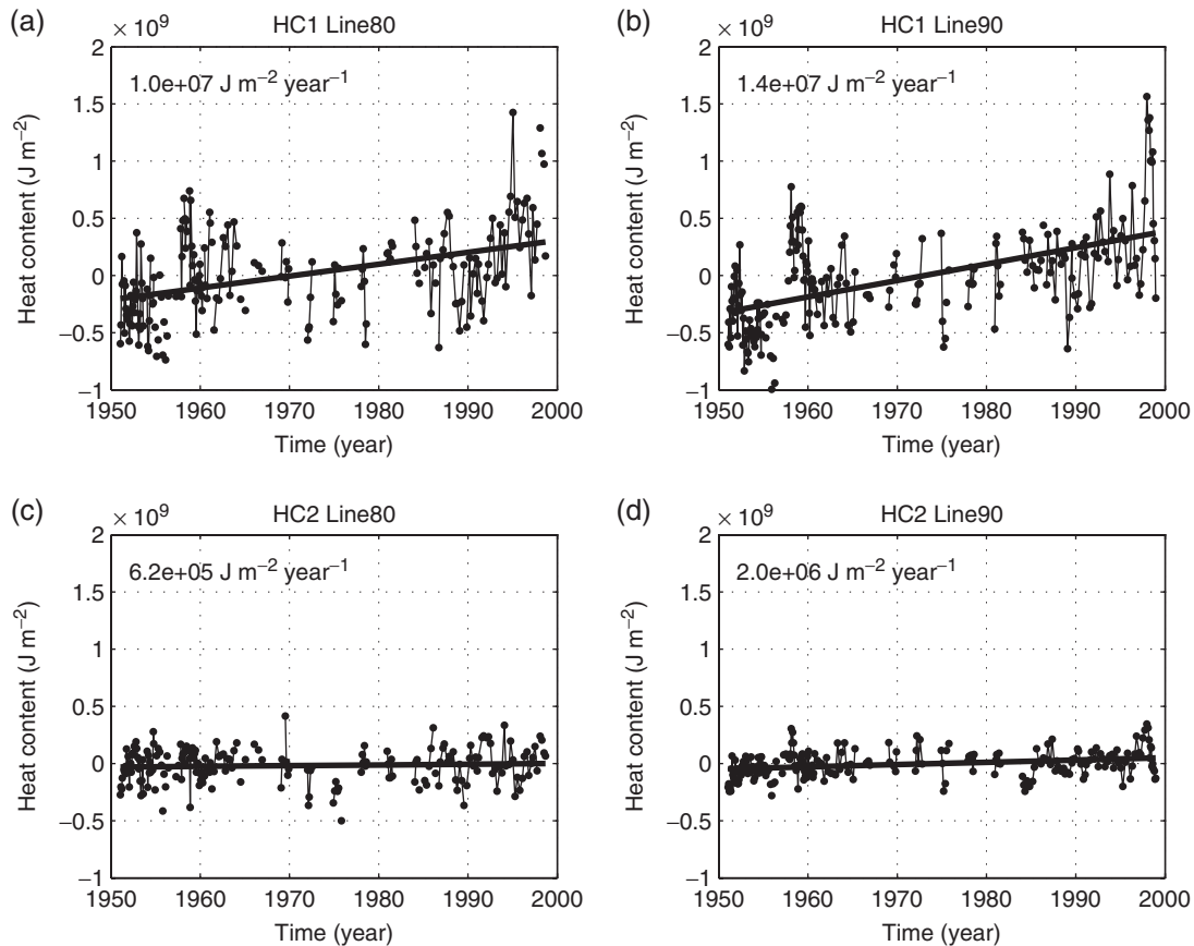
Fig. 5 Heat content anomalies for Line 80 (a, c) and Line 90 (b, d) in the upper layer (20–200 m, a, b) and lower layer (300–500 m, c, d). Upper-ocean heat content was defined as the vertical integral of \rho C_p T(z) , where \rho is the average seawater density ( 1025 \text{ kg m}^{-3} ), C_p is the heat capacity of seawater ( 3985 \text{ J kg}^{-1} \text{ K}^{-1} ), and T(z) is vertical temperature profile obtained by interpolating the temperature into 1 m vertical resolution. The upper layer has a stronger warming trend than the lower layer. HC1, heat content between 20 and 200 m; HC2, heat content between 300 and 500 m. Regression in (c) is not significant.
