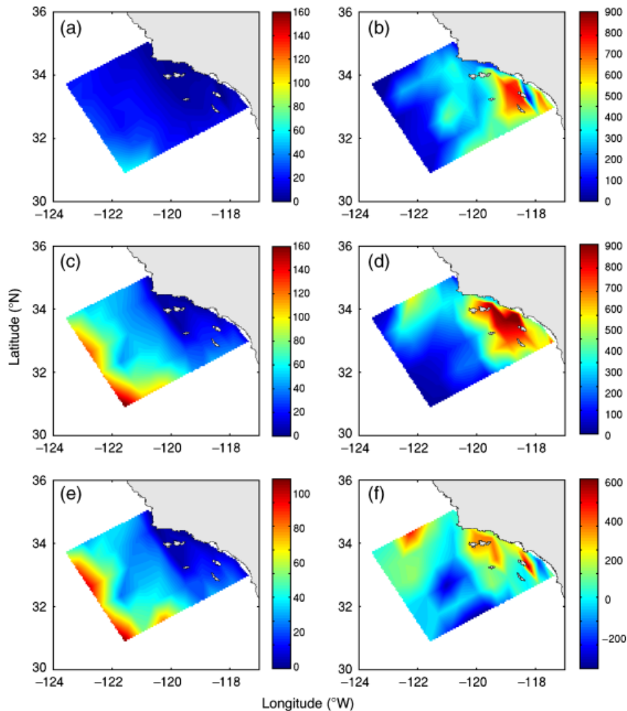
Fig. 8 Average abundance (individuals/10 m 2 ) maps of the oceanic and coastal-neritic species in the cold (a, b) and warm (c, d) period respectively, and the difference of the average abundances between the warm and cold period (warm – cold) for oceanic (e) and coastal-neritic group (f). For the oceanic group, only taxa with significantly higher abundance in the warm period were used, while for the coastal-neritic group, all taxa were used for calculation.
